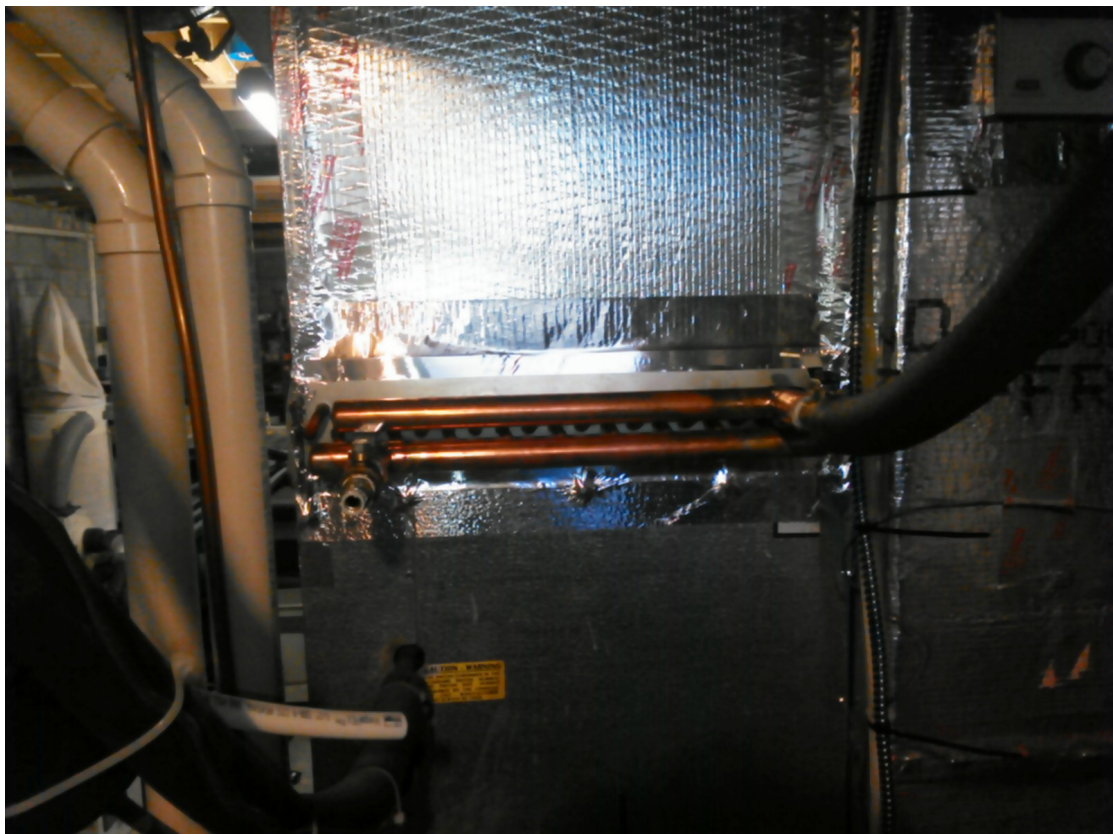
Manifold connections to underfloor heating from Microsolar on roof. Bassett Residence Sunbury PA.
